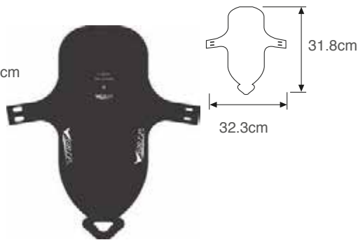
V-9988-XF Tablet Fender Material PP Thickness : 1.0mm
